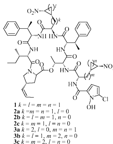
Figure 1. Structures of hormaomycin ( 1 ) and its analogues 2a–c and 3a–c .
